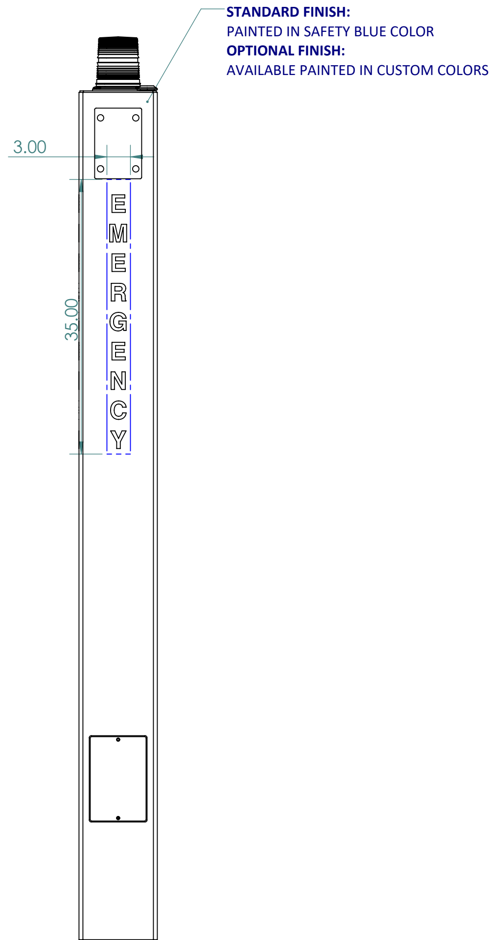
REAR VIEW
