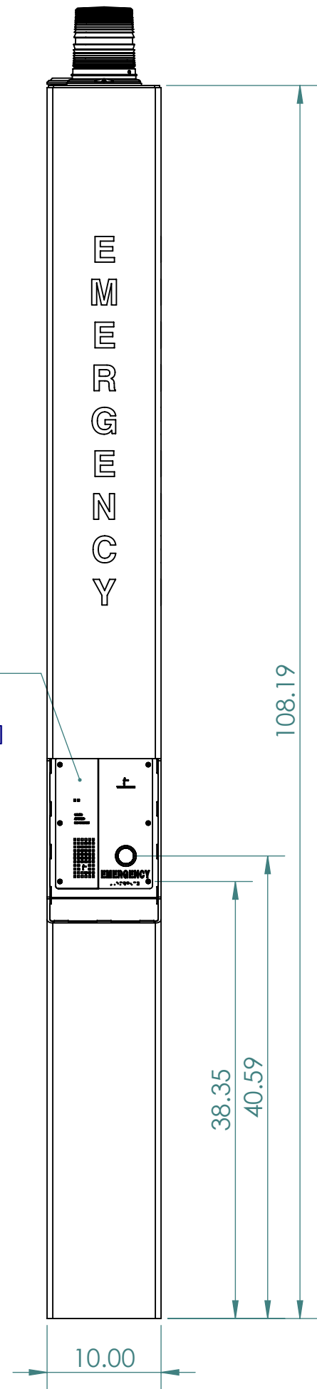
FRONT VIEW
