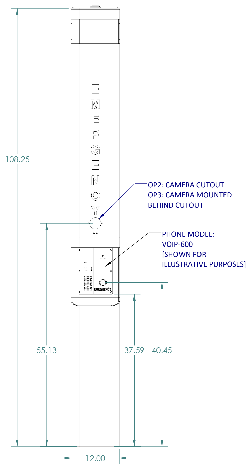
FRONT VIEW
