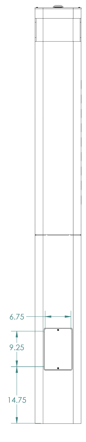
REAR VIEW
