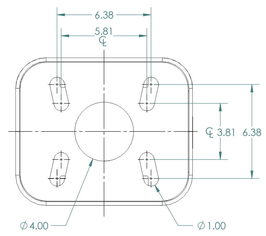
FOOT PRINT
